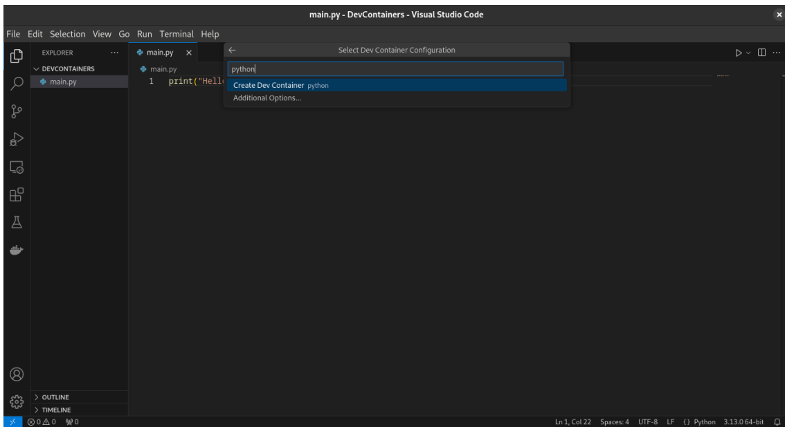
Figure 30.5: Create DevContainer
