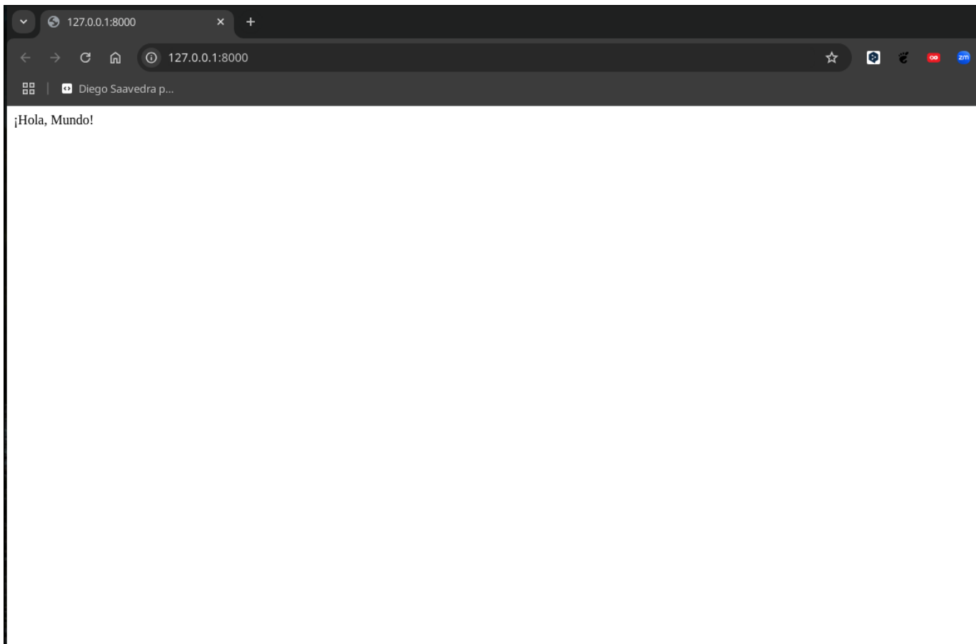
Figure 55.3: Django
