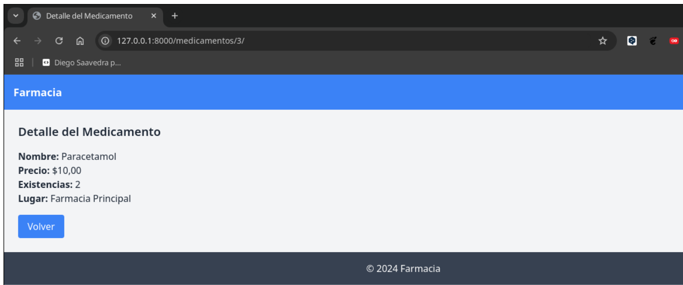
Figure 76.1: Django
