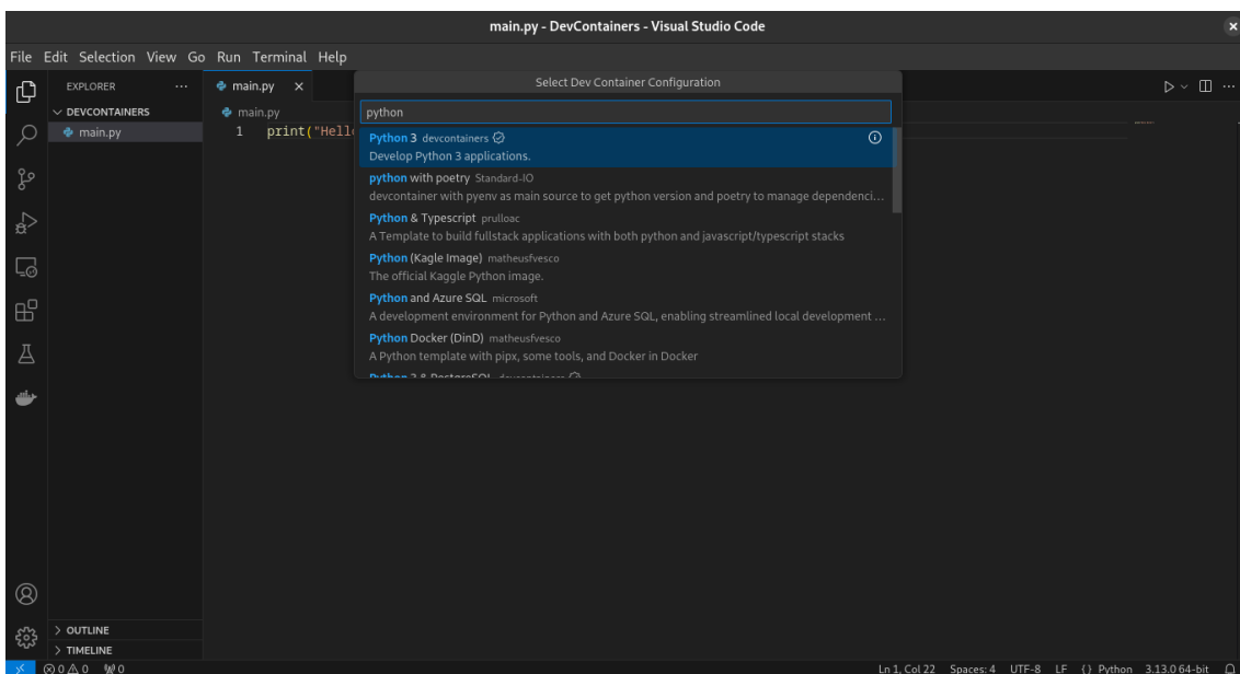
Figure 30.4: Python 3 DevContainer
