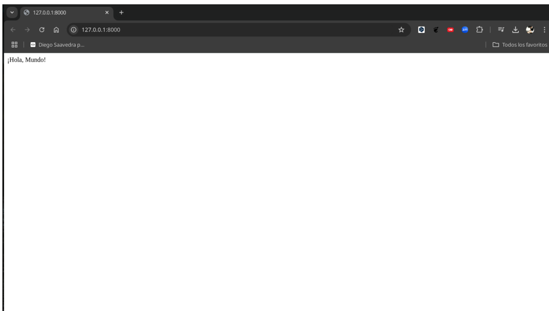
Figure 52.8: Django
