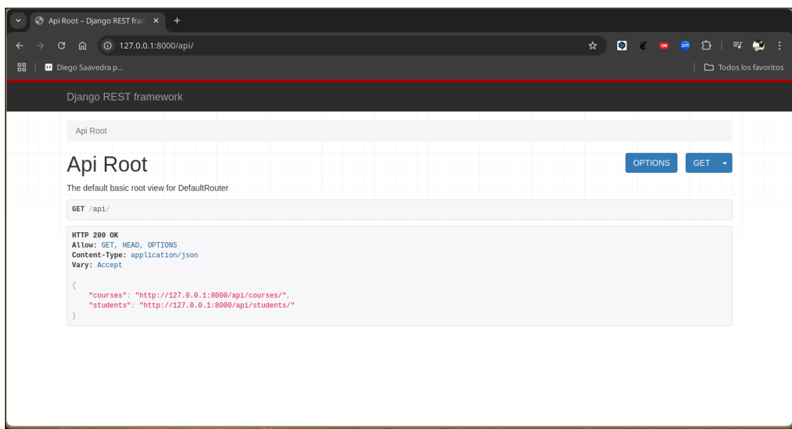
Figure 100.1: Django
