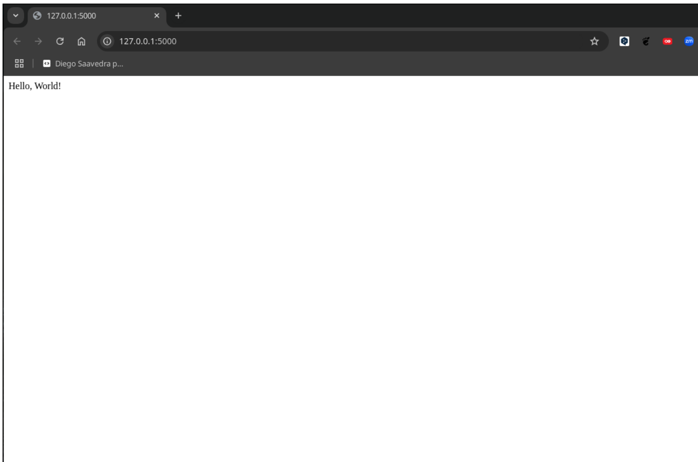
Figure 52.5: Flask
