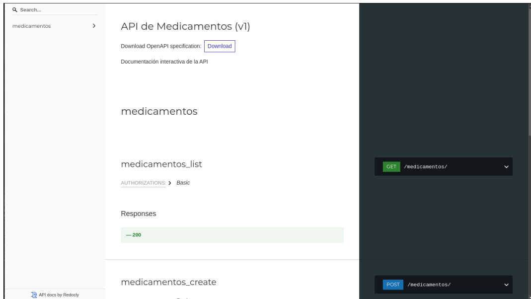
Figure 82.3: Redoc
