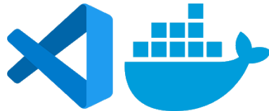
Figure 30.1: DevContainers
