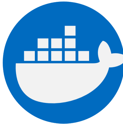
Figure 26.1: Docker
