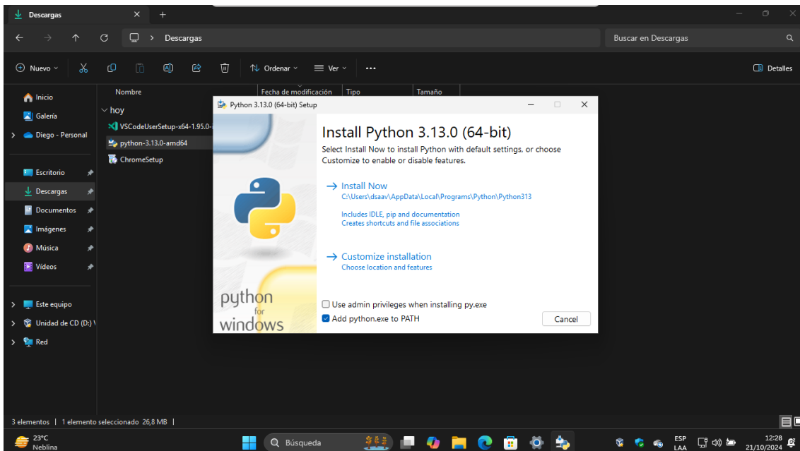
Figure 6.6: Python
