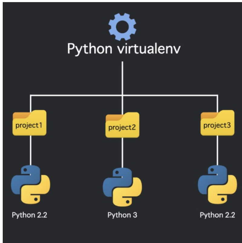
Figure 52.2: Entornos Virtuales
