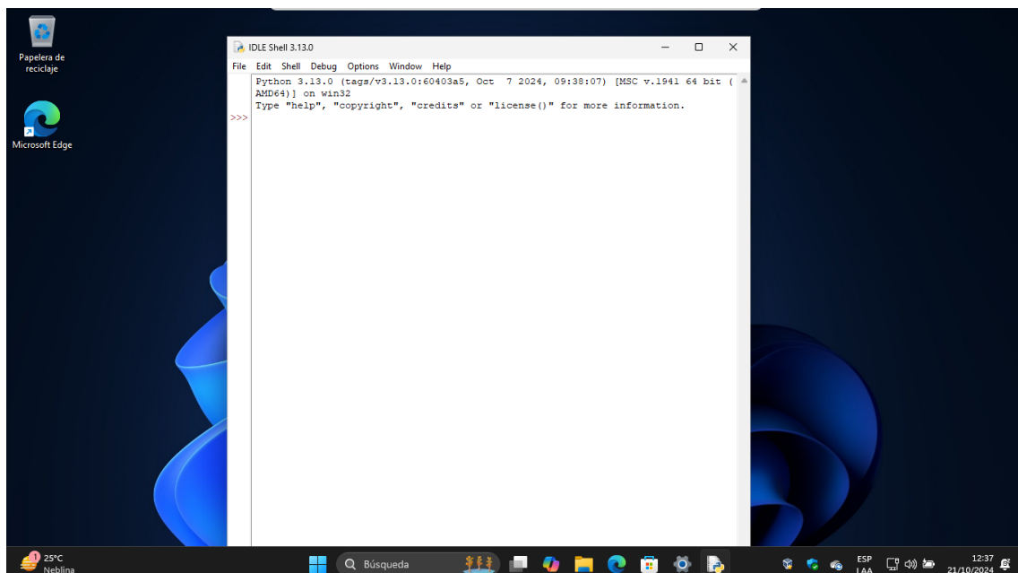
Figure 8.1: IDLE
