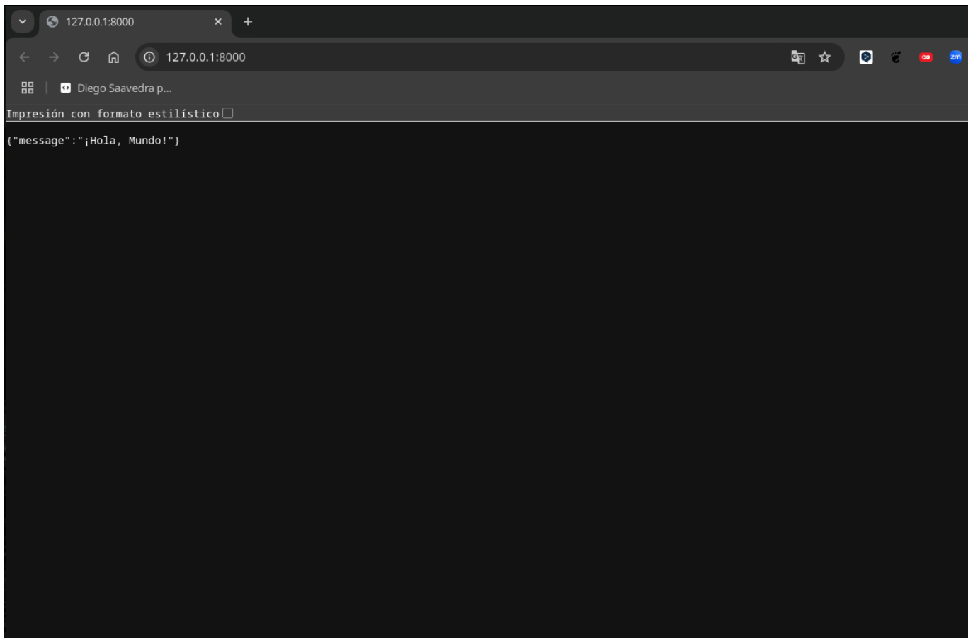
Figure 52.11: FastAPI
