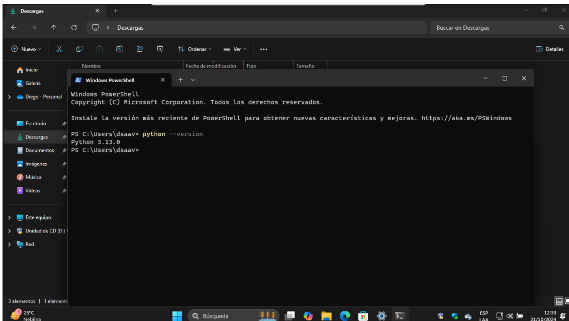
Figure 6.7: Python
