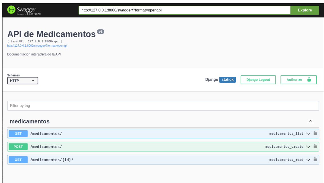
Figure 82.2: Swagger
