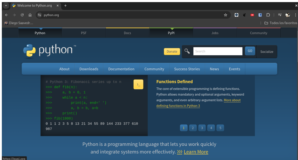
Figure 6.3: Python
