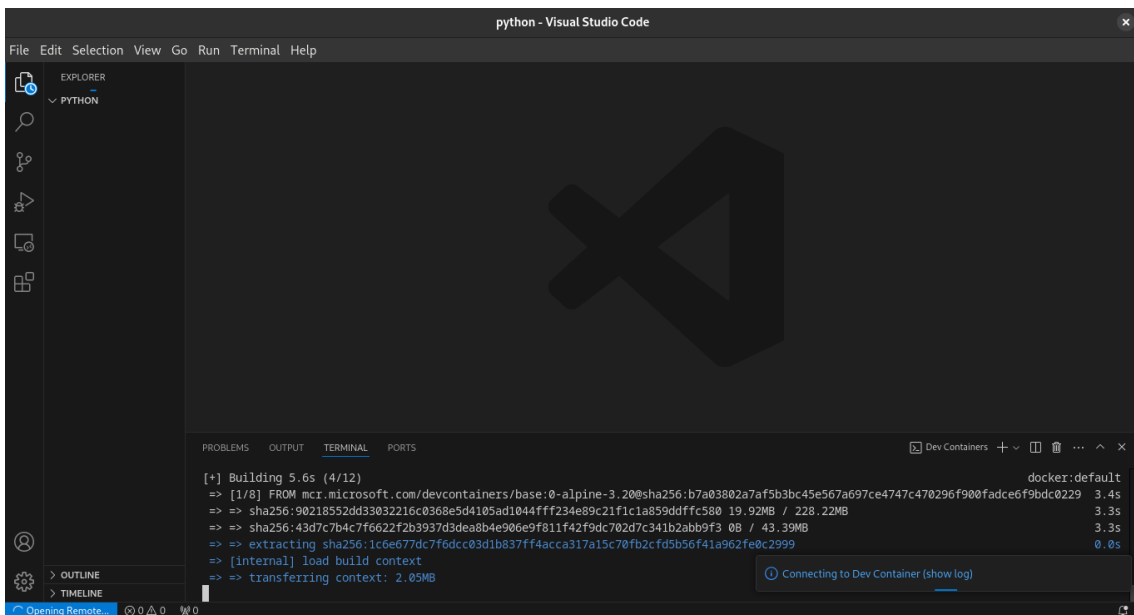
Figure 30.6: Create DevContainer
