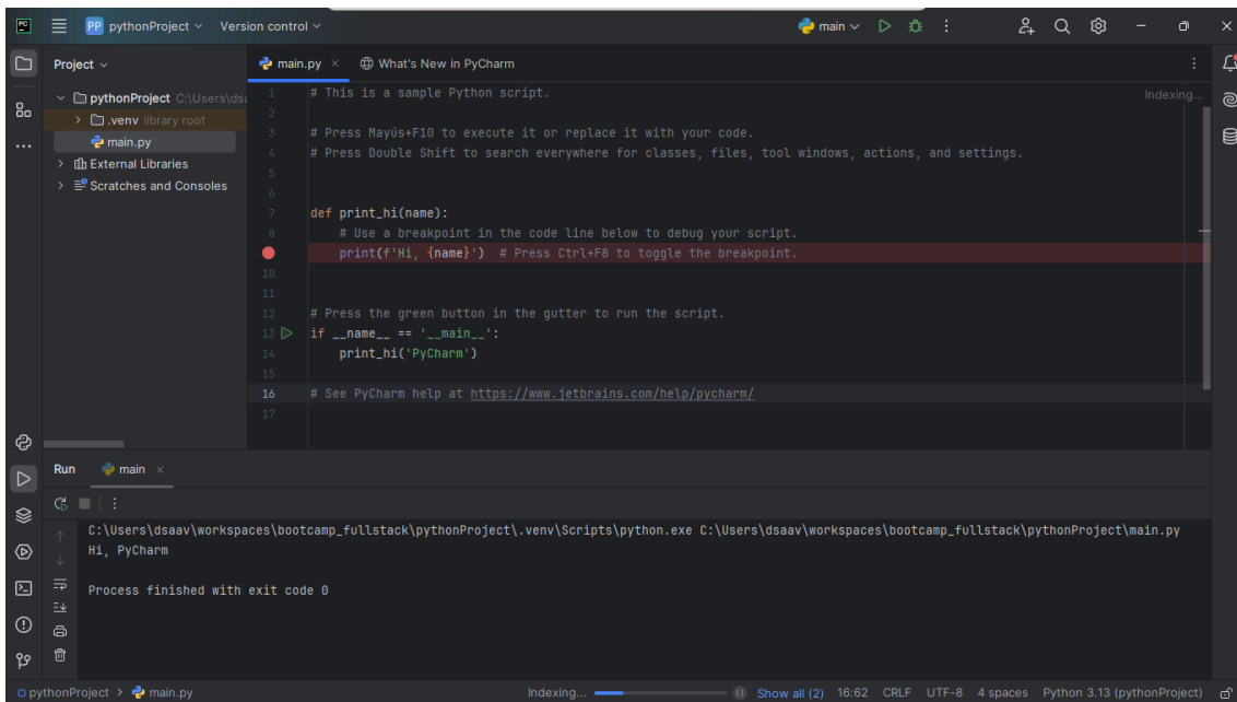
Figure 8.2: PyCharm
