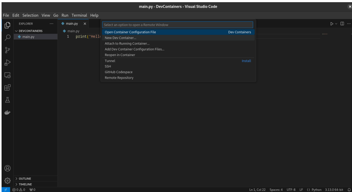
Figure 30.3: New DevContainer
