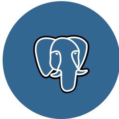
Figure 48.1: PostgreSQL Database
